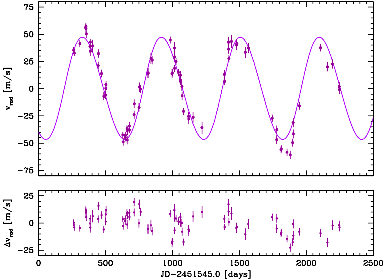
Fig. 1.— Top Panel: Radial velocities measured at Lick Observatory, along with error bars, covering about 5.5 years from September 2000 to February 2006. The best fit Keplerian is overplotted, with a period of 589.7 days. Bottom Panel: Radial velocity residuals after the best fit Keplerian has been subtracted. The remaining radial velocity scatter has a standard deviation of 9 m/s, and no systematics are visible in the residuals, neither by eye nor in the periodogram of the residuals in the lower part of Fig. 2.
