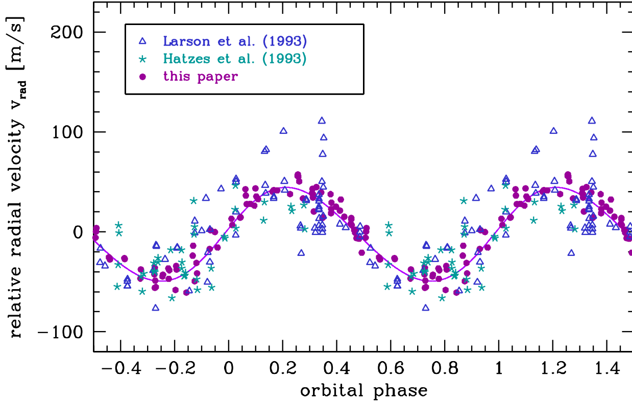
Fig. 3.— Radial velocities from Larson et al. (1993) (open triangles) and Hatzes & Cochran (1993) (asterisks) phased to the period determined from our own measurements (filled circles). Our orbital fit is also shown (solid line). No changes in period or amplitude of the periodic RV signal is apparent from that plot. For clarity, no individual error bars have been included in the plot. The data in Larson et al. (1993) consist of two separate datasets; data from CFHT have mean internal errors of 12 m/s, data from DAO 27 m/s. The majority of the datapoints in Hatzes & Cochran (1993) has mean internal errors of around 20 m/s, while a few datapoints have mean internal errors of 7 m/s. Note that not all of the measurements in Hatzes & Cochran (1993) have been used; the second set of 13 measurements in their Table 1C is identical to the first 13 measurements and thus obviously wrong, so it has been omitted. Errors for the DAO dataset from Larson et al. (1993) are rather inhomogeneous and reach up to around 80 m/s for some measurements, which explains the few data points which seem to be outliers in this graph.
