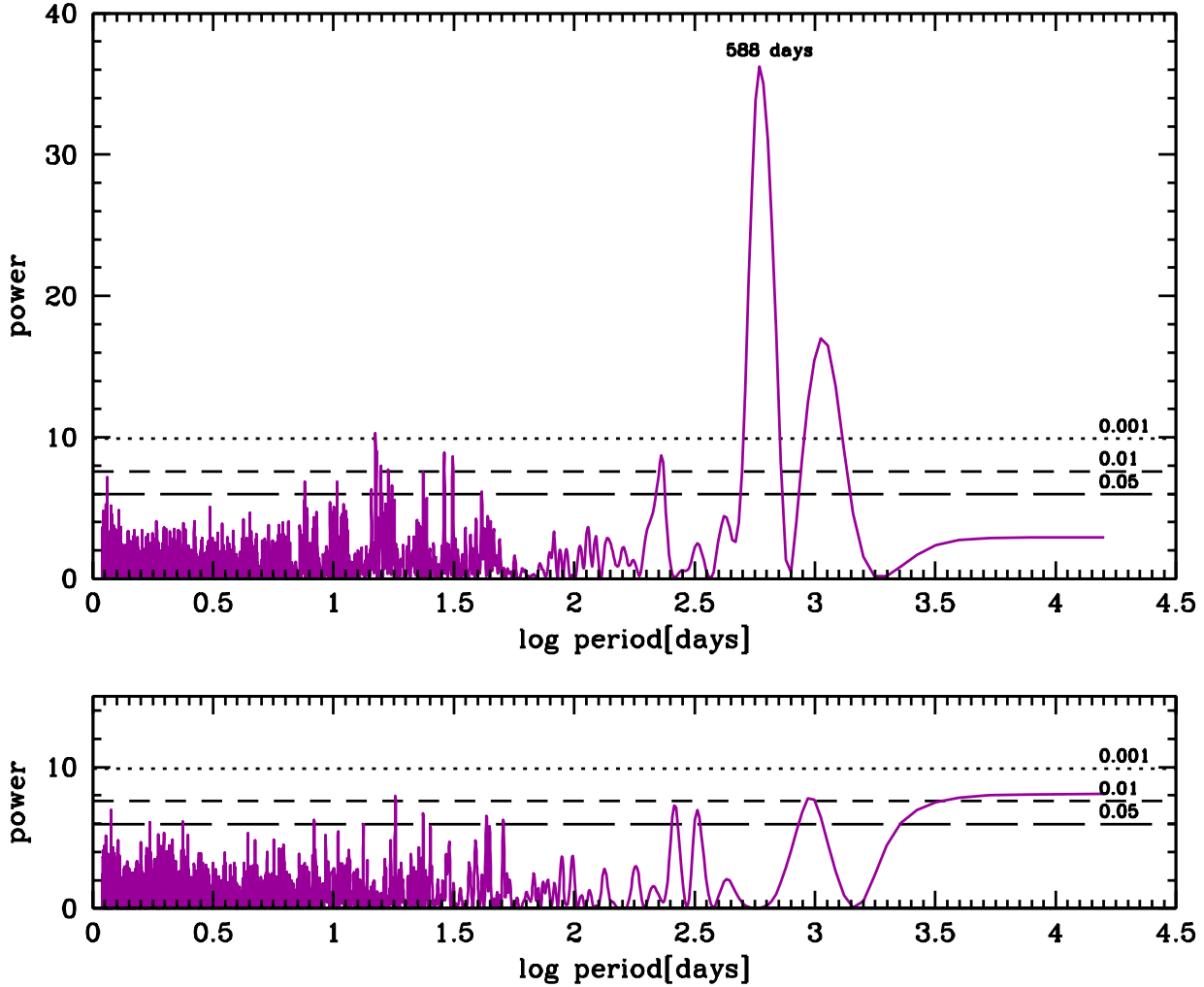
Fig. 2.— Top Panel: periodogram of the measured radial velocities. The highly significant peak occurs at 588 days; a Kepler fit to the data reveals a best fit period of 589.7 days. The next significant peak to the right, at about \log P[\text{days}]=3.07 , corresponds to twice the value of the most significant period. The numbers at the right indicate the false alarm probabilities of the labeled lines; a highly significant peak in the periodogram would sit clearly above the highest line, indicating a false alarm probability of less than 0.1%. Bottom panel: same as above, but with the Kepler fit corresponding to 589.7 days removed from the radial velocities. No significant peak is left in the periodogram of the radial velocity residuals.
