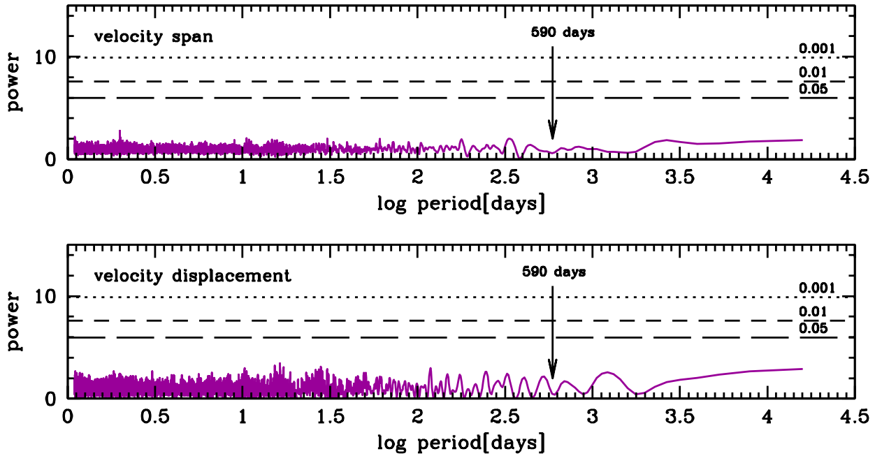
Fig. 4.— Periodograms of the derived bisectors. Top panel: velocity span, bottom panel: velocity displacement. There are no significant periodicities visible; all trial periods have an extremely small probability of being real. The period present in the RV data is indicated.
