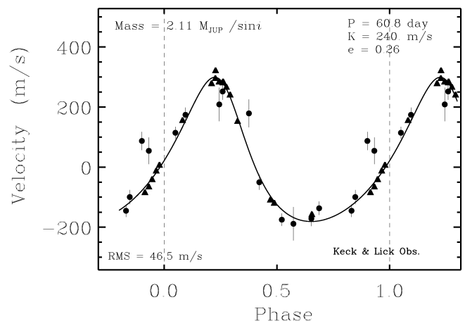
FIG. 3.—Combined Lick and Keck radial velocities for Gliese 876, plotted vs. orbital phase. Filled circles are from Lick, and the triangles come from Keck. The solid line is the radial velocity curve from the orbital solution.
