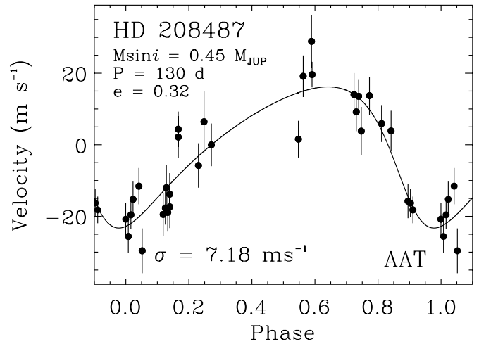
FIG. 9.—AAT Doppler velocities of HD 208487 from 1998 August to 2004 August phased to the period of the best-fit Keplerian orbit. The orbit is eccentric ( e = 0.32 ), with amplitude 20 \text{ m s}^{-1} , and the period is 130 days, resulting in a minimum mass ( M \sin i ) companion of 0.45M_{\text{JUP}} \pm 0.05M_{\text{JUP}} and semimajor axis of 0.49 \pm 0.04 \text{ AU} . The rms of the velocities about the fit is 7.2 \text{ m s}^{-1} .
