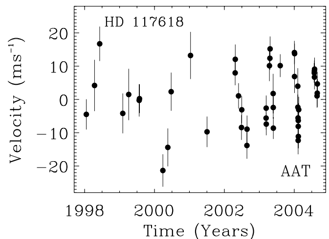
FIG. 4.—Measured velocities of HD 117618. The rms is 9.0 \text{ m s}^{-1} compared to the median internal measurement uncertainty of 4.1 \text{ m s}^{-1} and the expected level of stellar jitter of 2\text{--}4 \text{ m s}^{-1} .
