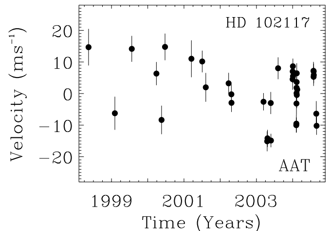
FIG. 10.—Measured velocities of HD 102117. The rms is 8.26 \text{ m s}^{-1} compared to the median internal measurement uncertainty of 3.2 \text{ m s}^{-1} and the expected level of stellar jitter of 2\text{--}4 \text{ m s}^{-1} .
