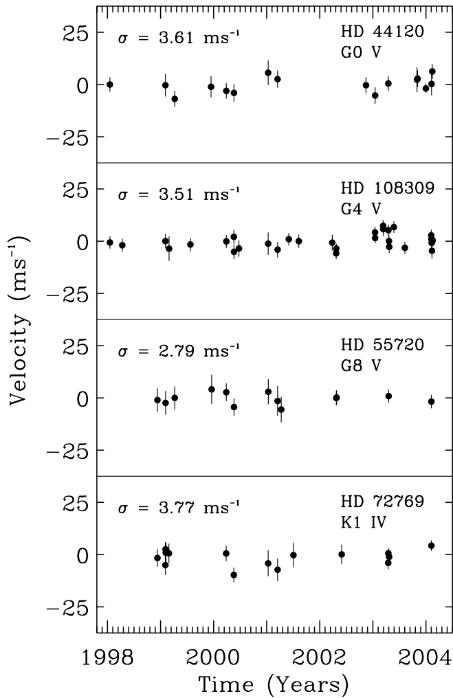
FIG. 1.—Four chromospherically quiet stars with B - V and spectral types similar to the planet-bearing stars presented in this paper. The long-term single-shot precision of the AAPS is 2\text{--}3\text{ m s}^{-1} for suitable inactive stars.
