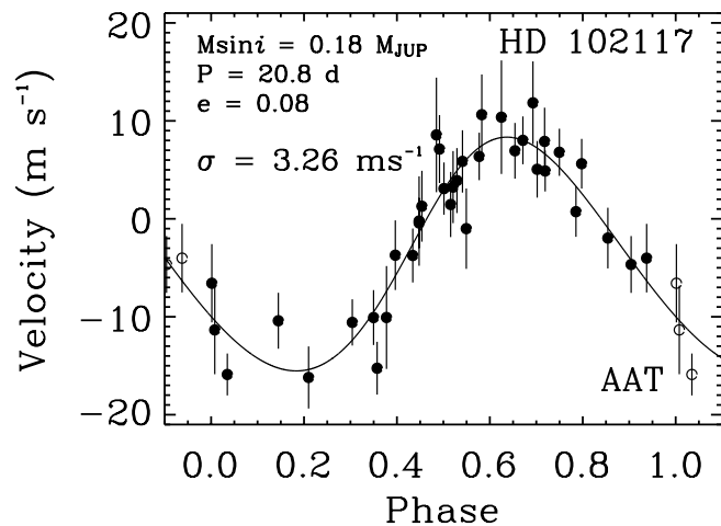
FIG. 12.—AAT Doppler velocities for HD 102117 from 1998 May to 2004 August, phased at the best-fit Keplerian period of 20.8 days. The orbit is nearly circular ( e = 0.08 ), and the amplitude is 12 \text{ m s}^{-1} . The resultant minimum mass ( M \sin i ) of the companion is 0.18M_{\text{Jup}} \pm 0.03M_{\text{Jup}} with a semimajor axis of 0.15 \pm 0.01 \text{ AU} . The rms of the velocities about the fit is 3.3 \text{ m s}^{-1} .
