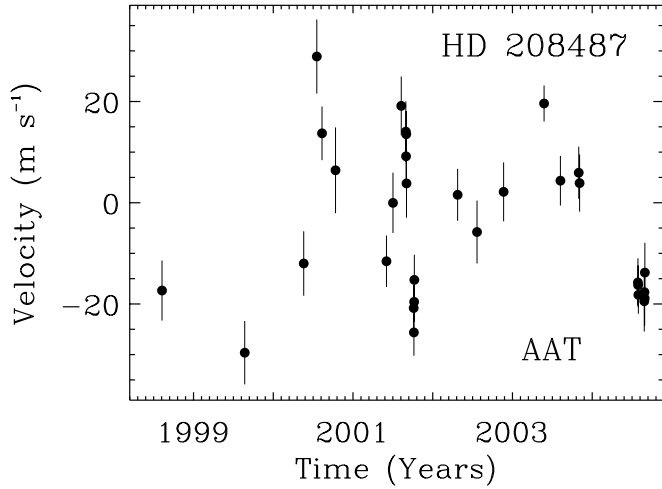
FIG. 7.—Measured velocities of HD 208487. The rms is 15.3 \text{ m s}^{-1} compared to the median internal measurement uncertainty of 5.1 \text{ m s}^{-1} and the expected level of stellar jitter of 2\text{--}4 \text{ m s}^{-1} .
