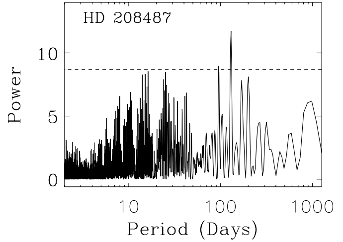
FIG. 8.—Periodograms of the 31 observations of HD 208487 obtained at the AAT between 1998 August and 2004 August. The dashed line is the 0.1% false-alarm level.
