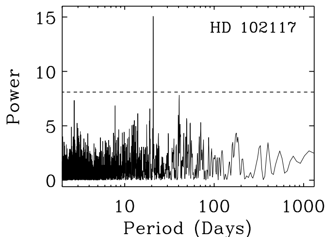
FIG. 11.—Periodogram of HD 102117 velocities. The dotted lines shows the 0.1% false-alarm level. The single dominant period is at 20.8 days.
