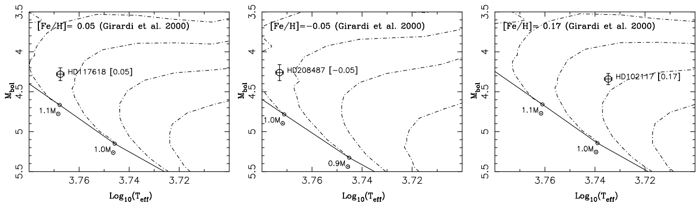
FIG. 2.—Evolutionary tracks from the compilation of Girardi et al. (2000), interpolated to the estimated metallicities for stars under discussion in this paper. The zero-age main sequence is shown as a solid line, with evolutionary models at the indicated masses shown as dot-dashed lines. The open circles and uncertainties indicate the stars, with their estimated metallicities indicated in brackets.
