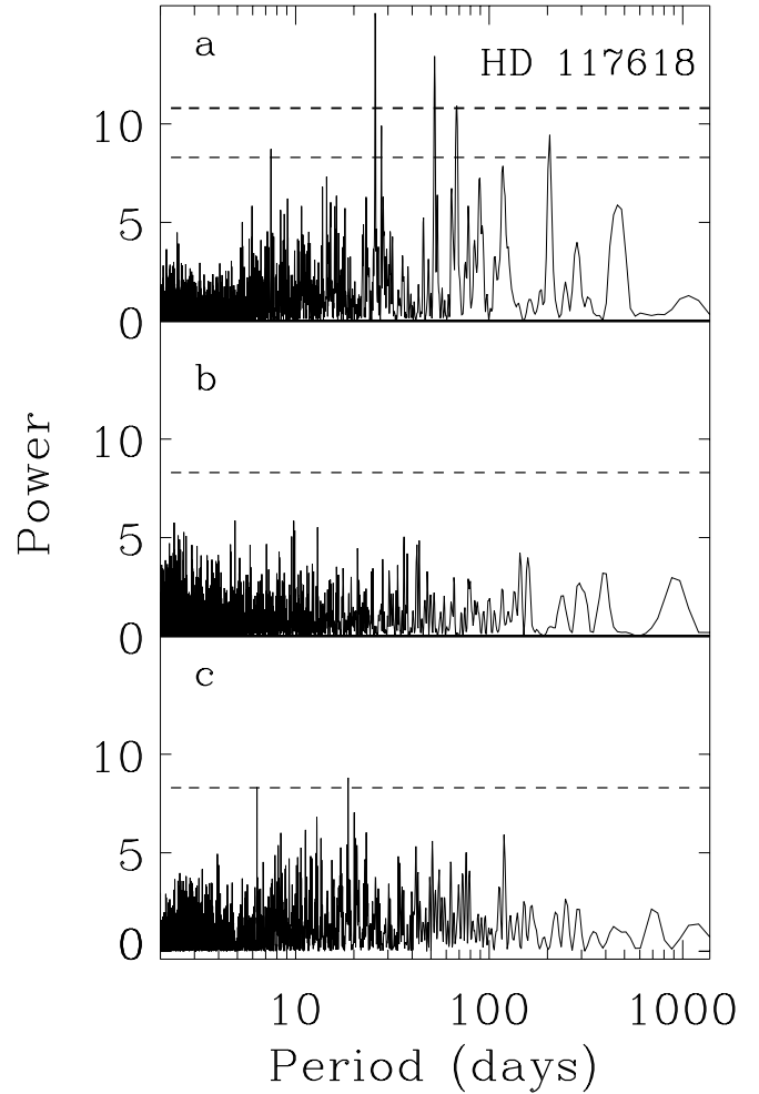
FIG. 5.—Periodograms of the 47 observations of HD 117618 obtained at the AAT between 1998 January and 2004 August. The false alarm probabilities provided are based on the assumption of normally distributed errors. (a) Periodogram of all velocities. The top dashed line is the 0.1% false alarm level, while the bottom dashed line is the 1% false alarm level. The two highest peaks are at the two possible periods of 25.8 and 52.2 days. (b) Periodogram of velocity residuals after removing the best-fit Keplerian with a period of 25.8 days. The dashed line is the 1% false alarm level. (c) Periodogram of velocity residuals after removing the best-fit Keplerian with a period of 52.2 days. The dashed line is the 1% false-alarm level.
