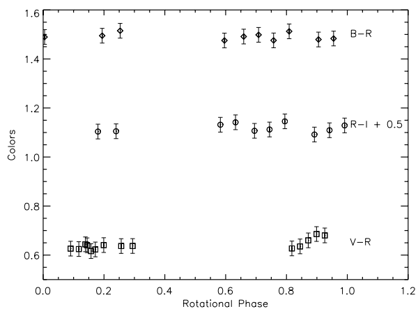
FIG. 5.— B – R , R – I , and V – R colors of Varuna, showing no significant variation over its rotation. The R – I colors have been shifted up by 0.5 mag for clarity in distinguishing them from the V – R colors.
