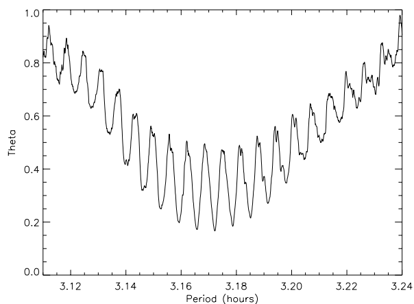
FIG. 3.—Same as Fig. 2, but with period as the x -axis and at higher resolution on the single-peaked best fit, to show the aliases caused by the \sim 60 day gap between the February and April observations. The three lower peaks are all reasonable fits to the data, with the middle peak at 3.1721 hr being the best fit for the single-peaked light curve.
