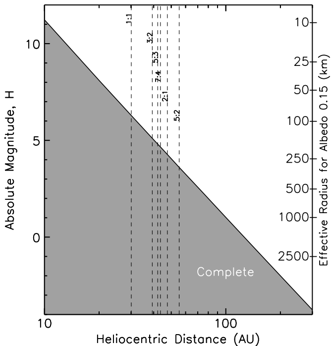
Figure 7. Heliocentric distance versus the completeness of absolute magnitude, H. The shaded region shows where the outer solar system should be complete in discoveries. The effective radius on the right side assumes an albedo of 0.15. The average semi-major axis for the various major Neptune resonance populations is shown as vertical dashed lines for reference.
