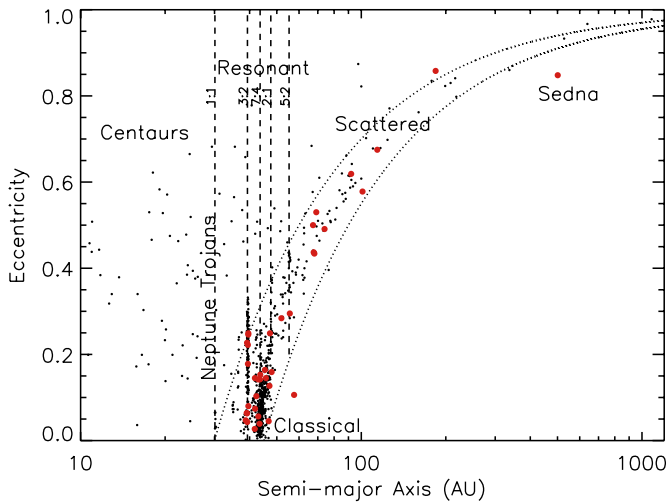
Figure 10. Semi-major axis vs. eccentricity of multi-opposition trans-Neptunian objects. Large circles represent TNOs with H \leq 4.5 mag. This figure shows several distinct dynamical KBO populations. Vertical dashed lines show the main resonances with Neptune as well as the Neptune Trojans in the 1:1 resonance. Scattered disk objects have perihelia 30 \lesssim \text{peri} \lesssim 45 AU as shown between the dashed lines. Classical objects are in the lower center portion of the figure and include the main Kuiper Belt (MKB) with its high and low inclination populations. There also appears to be a high and low eccentricity population of large objects. An edge near 50 AU can clearly be seen for low eccentricity objects. Centaurs are on unstable orbits between the giant planets. Sedna stands out as being significantly below the perihelion line shown at 45 AU demonstrating its decoupled influence from Neptune unlike the scattered disk objects.
