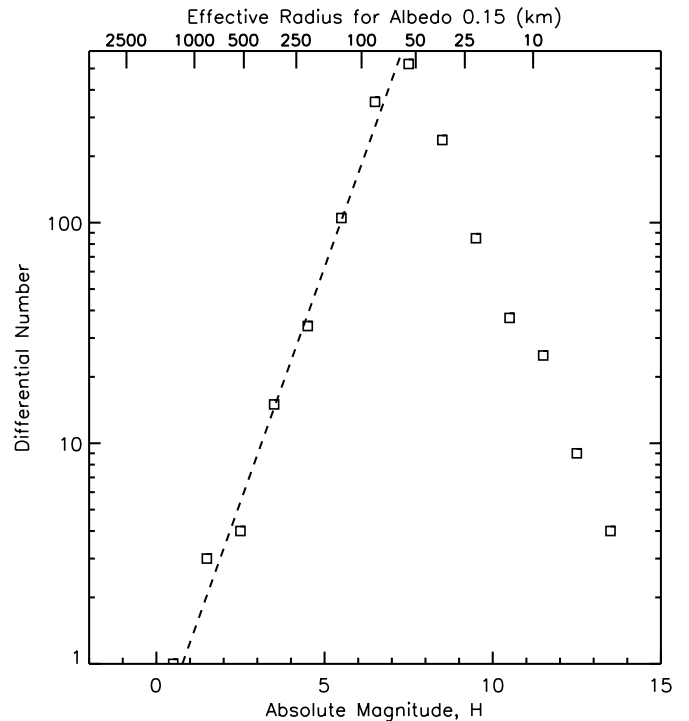
Figure 9. Absolute magnitude vs. the differential number of known trans-Neptunian objects. Objects are binned in 1 mag bins. The largest few objects have had their absolute magnitudes adjusted fainter as in Figure 8 to account for their higher albedos compared to the smaller objects. The dashed line shows the best fit to the largest objects. It is apparent that the Kuiper Belt is nearly complete to about an absolute magnitude of around 5–6 mag after which a turnover shows significant incompleteness.
