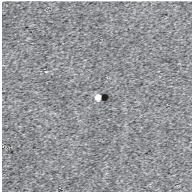
Figure 4. Difference image of the Pluto fields (Figure 3) showing the removal of the steady-state background of stars. The motion of Pluto is clearly revealed in the difference image as a positive (bright) and negative (dark) point from the subtraction process of the two individual images.
