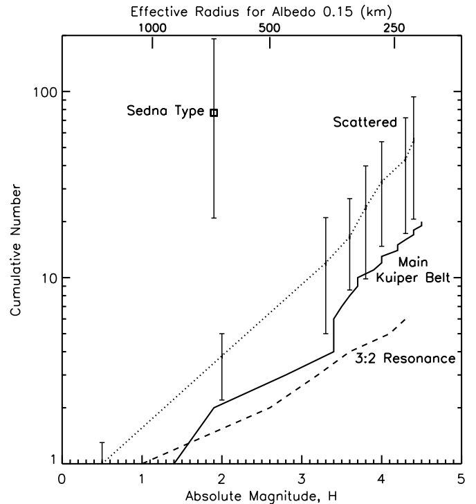
Figure 11. Absolute magnitude vs. the cumulative number of objects for the various completeness limits (see Table 4) of the dynamical classes in the Kuiper Belt. The largest few objects have had their absolute magnitudes adjusted as in Figure 8 to account for their higher albedos compared to the smaller objects. The Sedna type (square) and scattered disk objects (dotted line) have significant error bars as these populations are not complete for even the largest objects. Poisson statistics were used to extrapolate the total scattered disk and Sedna populations from the known objects brighter than 21st magnitude using the amount of time the objects would be detectable in their eccentric orbits (Table 4). The scattered population is likely larger than either the main Kuiper Belt (solid line) or the 3:2 resonance population (dashed line). The Sedna type population appears to be the largest of all the populations by a factor of ten or more. The 3:2 resonance population has a shallower size distribution slope ( q = 2.2 \pm 0.5 ) than the other populations ( q = 3.3 \pm 0.7 ).
