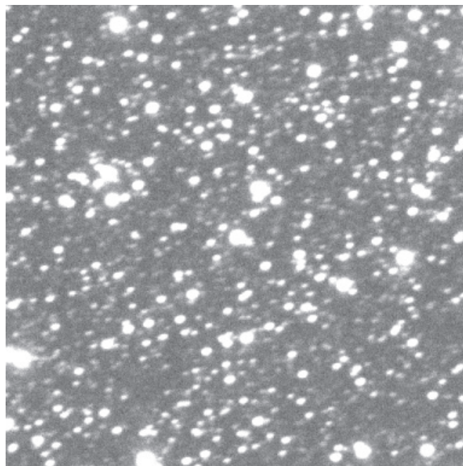
Figure 3. Small portion of an image showing Pluto in the Galactic Plane from the 1.3 m Warsaw telescope. Pluto is in the center of this image as revealed in Figure 4.
