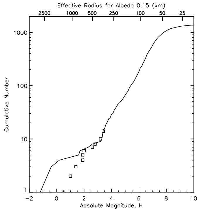
Figure 8. Absolute magnitude vs. the cumulative number of all known trans-Neptunian objects (solid line). The absolute magnitudes for the largest objects appear overly bright since these objects have much higher albedos than most smaller KBOs. Squares show the absolute magnitudes that the largest KBOs would have if their albedos were 0.15 and not around 0.7 as has been found for Eris, Pluto, Makemake, and Haumea. Squares also show the absolute magnitudes the moderately sized KBOs would have if their albedos were not around 0.25 but 0.15 for Sedna, 2007 OR10, Orcus, and Quaoar (Stansberry et al. 2008).
