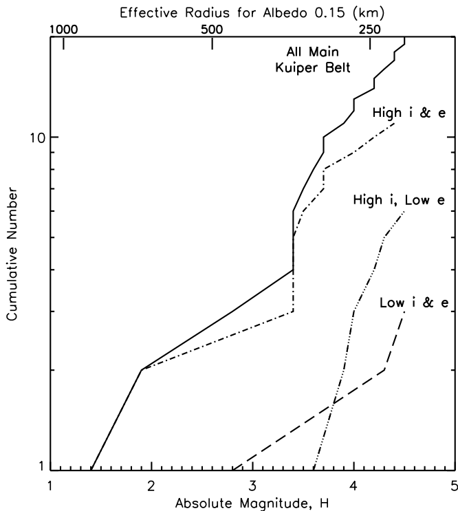
Figure 12. Absolute magnitude vs. the cumulative number of objects in the main Kuiper Belt (solid line) and its subcategories. The largest few objects have had their absolute magnitudes adjusted as in Figure 8 to account for their higher albedos compared to the smaller objects. The high inclination ( i > 10^\circ ) and eccentricity ( e > 0.13 ) objects (dot-dashed line) dominate the main Kuiper Belt on the large end. There appears to be a sizable group of main Kuiper Belt objects that have high inclinations but low eccentricities ( e < 0.07 ) (triple dot-dashed line). These high i and low e objects could be related to either of the other subcategories in this figure. Large low inclination and low eccentricity objects (long dashed line) are very rare with only Quaoar being brighter than an absolute magnitude of 4.2.
