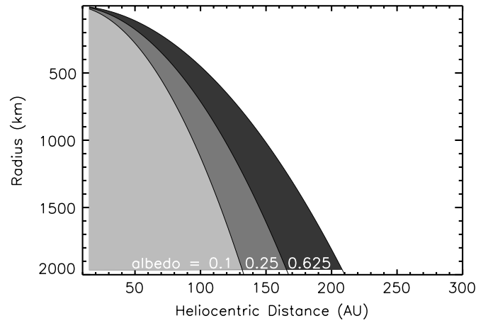
Figure 5. Outer solar system has now been surveyed to a completeness limit of about 21 mag in the R band. This figure shows what size and distance an object would be for several different albedos for a 21st magnitude object. Shaded areas correspond to completeness limits for albedo < 0.1 (light), albedo < 0.25 (medium), and albedo < 0.625 (dark). It is clear that a Pluto (1161 km) or even larger sized object could easily have gone undetected to date if beyond a few hundred.
