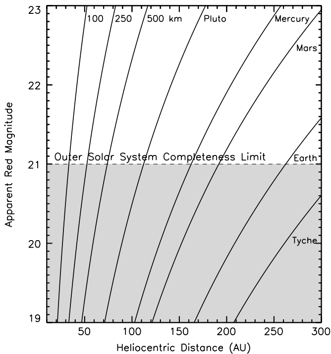
Figure 6. Radius of an object is shown assuming a moderate albedo of 0.15 for various heliocentric distances and apparent red magnitudes. The known objects in the Kuiper Belt region are complete to about 21st magnitude, shown by the shaded region below the dashed line. It is likely that everything under the dashed line at 21 mag is known. The radii used for the named objects in the figure are Pluto (1161 km), Mercury (2440 km), Mars (3396 km), Earth (6371 km), and an arbitrary lower limit on a hypothetical eccentric giant planet or companion to our Sun, sometimes called Nemesis or Tyche, with 10,000 km radius (Iorio 2009; Melott & Bambach 2010). In the distant solar system very large objects would easily be undetected to date.
