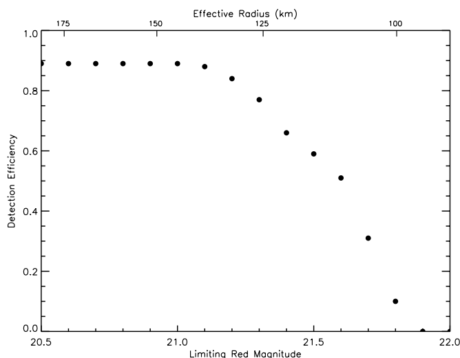
Figure 2. Detection efficiency of the KBO survey vs. the apparent red magnitude using the Warsaw 1.3 m telescope. In good seeing (0.8 arcsec FWHM) the 50% detection efficiency is at about 21.6 mag, while in moderate seeing ( \sim 1 arcsec) it is about 21.2 mag in the R band. Effective radii of the apparent magnitudes were calculated assuming the object has an albedo of 0.15 and is at 40 AU.
