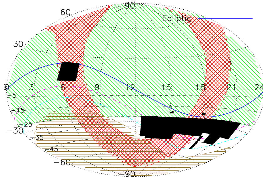
Figure 1. Black shaded regions represent the sky area surveyed in this work. The horizontal axis is the right ascension in hours and the vertical axis is the declination in degrees. The blue solid line shows the ecliptic, the magenta dashed line shows -20^\circ from the ecliptic, and the cyan dotted dashed line shows -30^\circ from the ecliptic. Areas more than -40^\circ south of the ecliptic are shown with brown horizontal stripes. The area within 15^\circ of the Galactic Plane is shown with red crossed stripes while the area covered by wide-field KBO surveys from the north (Trujillo & Brown 2003; Brown 2008; Schwamb et al. 2009, 2010) is shown with green angled stripes. Almost all KBOs are expected to be within 20^\circ of the ecliptic with it highly unlikely any KBO is beyond 40^\circ from the ecliptic (Brown 2008).
